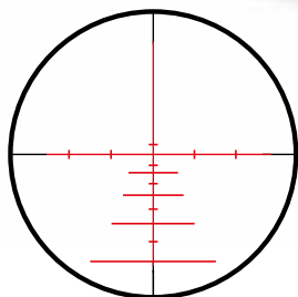
#7291 3x-12x44 ZOOM ENGRAVED 550 BALLISTIC WITH DUAL ILLUMINATION (RED-BLUE)
